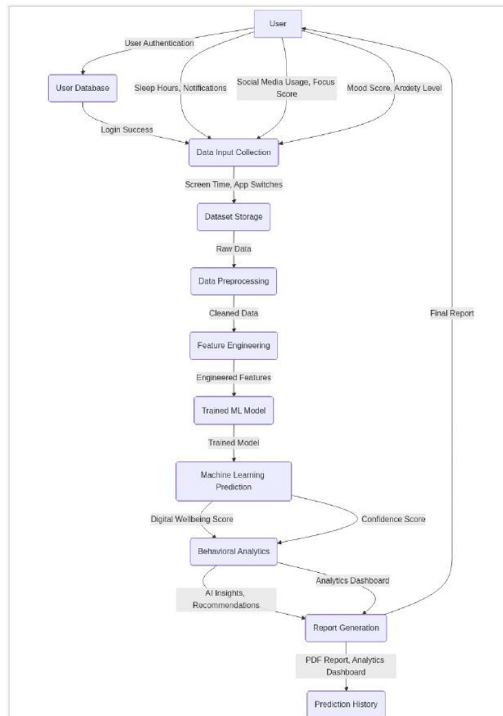
Fig 3.3:Data Flow Diagram
